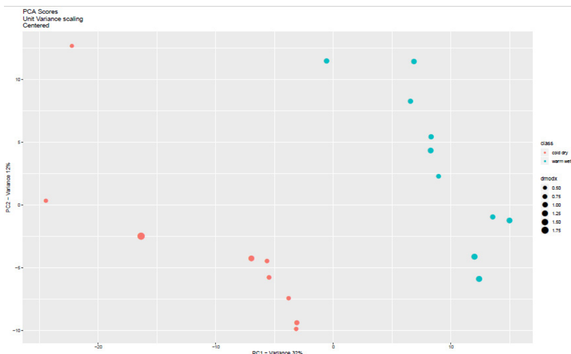
Figure 2. Principal component analysis (PCA) scores plot showing separate clusters for hot-wet and cold-dry temperaments.
